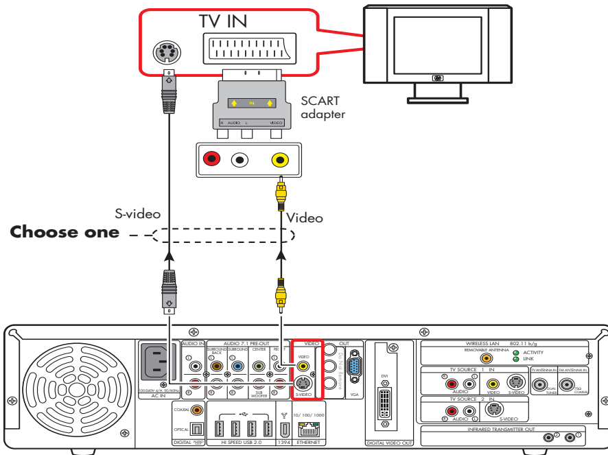
Video out to standard TV
